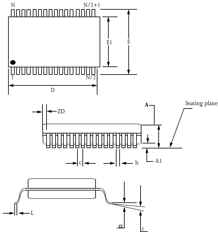
32-pin TSOP 2
