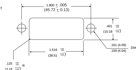
Dimensions for Rear Panel Mounting
