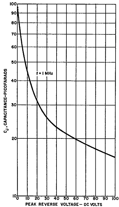
JUNCTION CAPACITANCE
