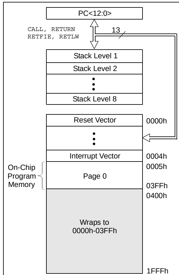
FIGURE 2-1: PROGRAM MEMORY MAP AND STACK FOR PIC16F818
