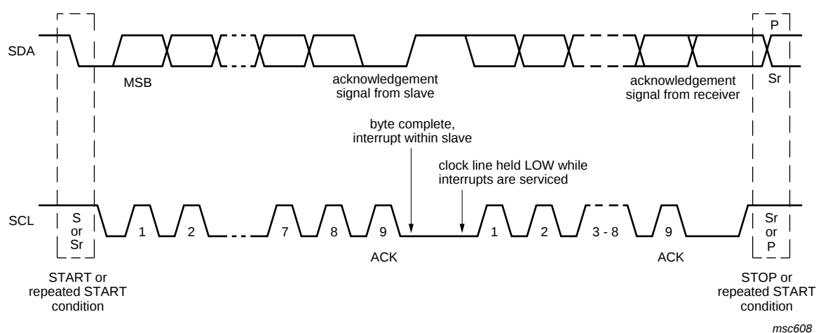
Fig 21. Data transfer on the I²C-bus
