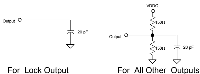
Figure 3. Output Waveforms
