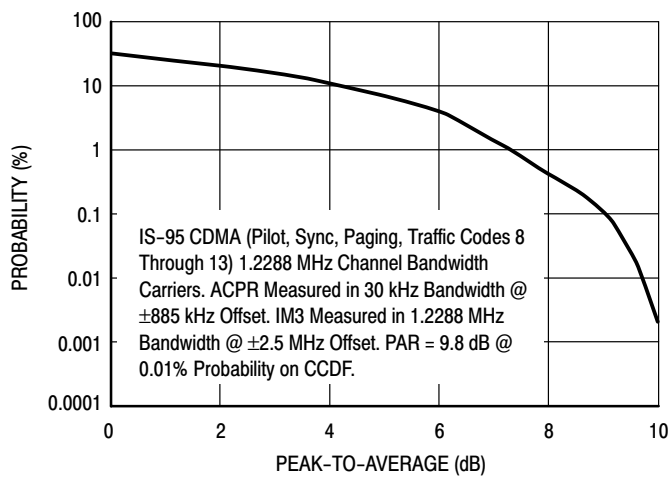
Figure 10. 2-Carrier CCDF N-CDMA
