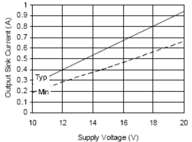
Figure 25. Output sink current vs. Voltage
