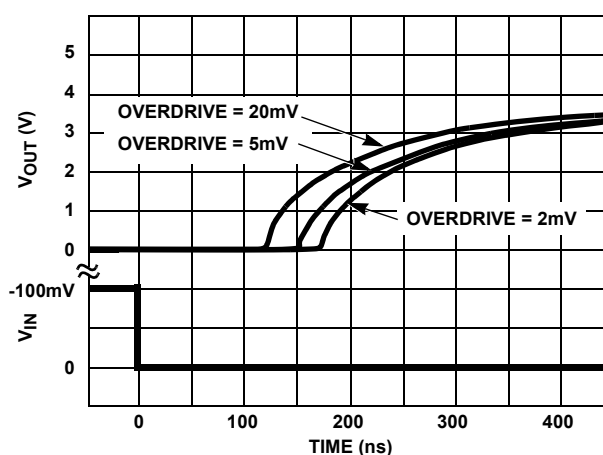
FIGURE 6. RESPONSE TIME FOR VARIOUS INPUT OVERDRIVES
