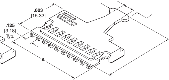
Cover 103058 Series with Cable Tie Paddle
