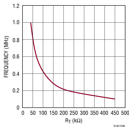
Figure 8. Frequency vs R_T Resistance
