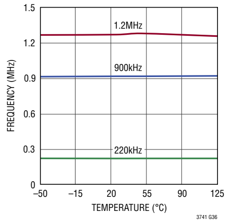
Oscillator Frequency
