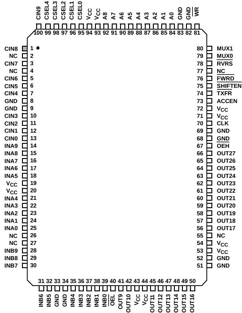
100 LEAD MQFP TOP VIEW
