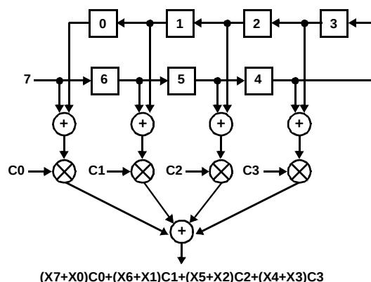
FIGURE 7A. DATA FLOW AS DATA SAMPLE 7 IS CLOCKED INTO THE FEED FORWARD STAGE
