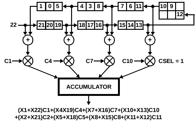
FIGURE 17B. COMPUTATIONAL FLOW AS DATA SAMPLE 22 IS CLOKED INTO THE FEED FORWARD STAGE
