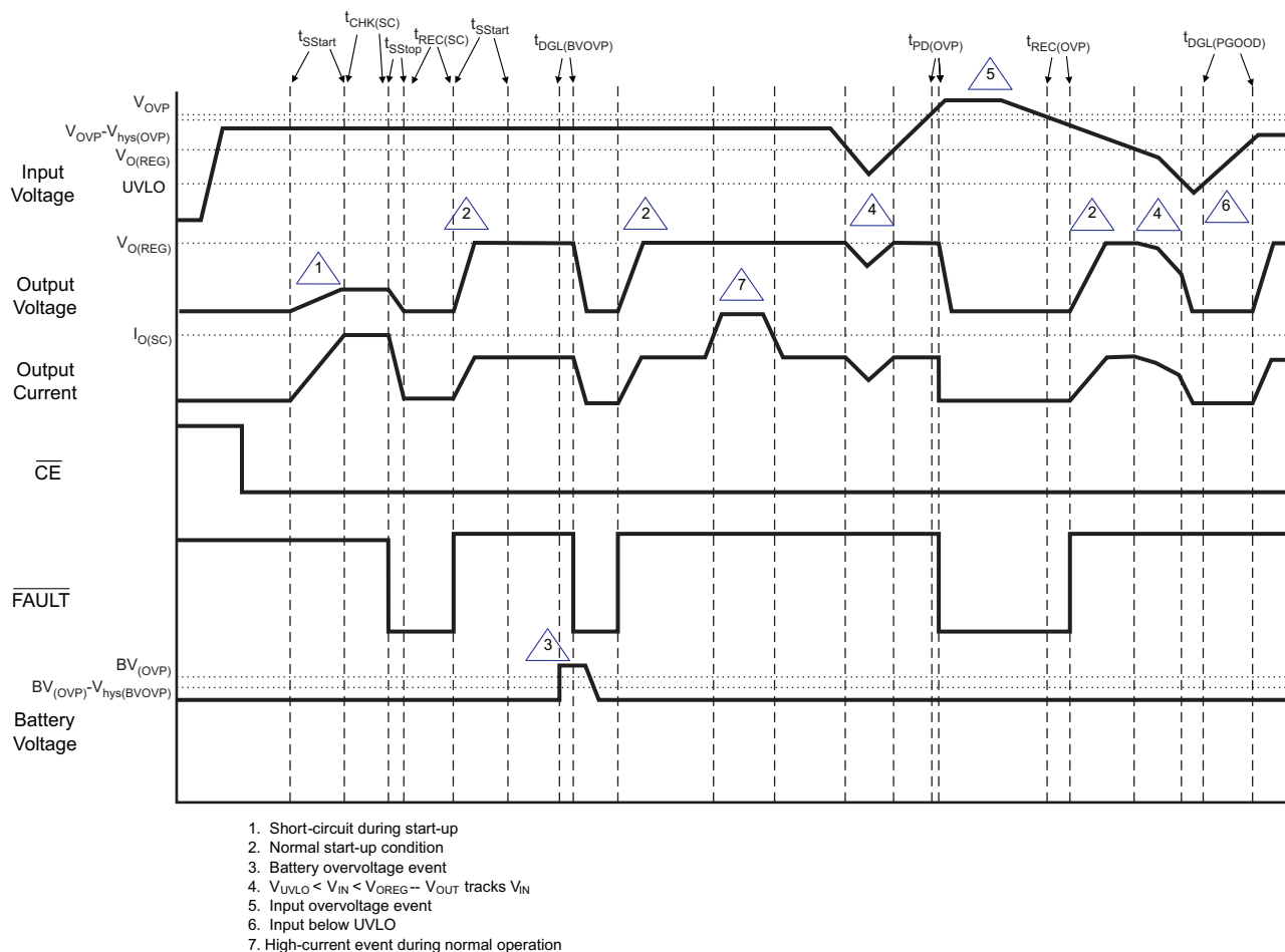
Figure 18. Timing Diagram
