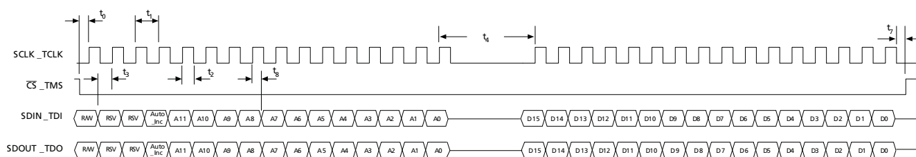
Figure 4-36: Write Mode
