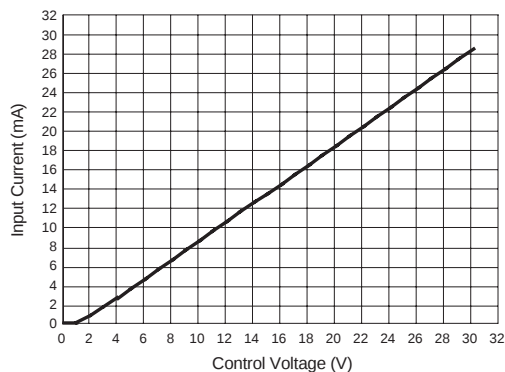
Figure 2 — G relays
