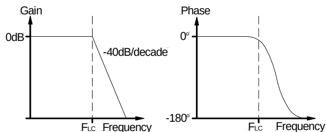
Figure 8 - Gain and phase of LC filter.
