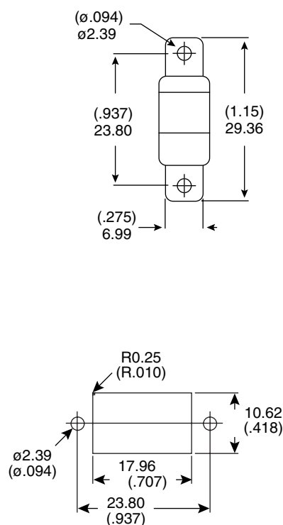
RECOMMENDED MOUNTING
