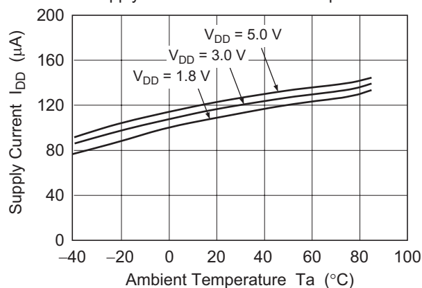
Figure 2-2. HA1630Q02 Supply Current vs. Ambient Temperature
