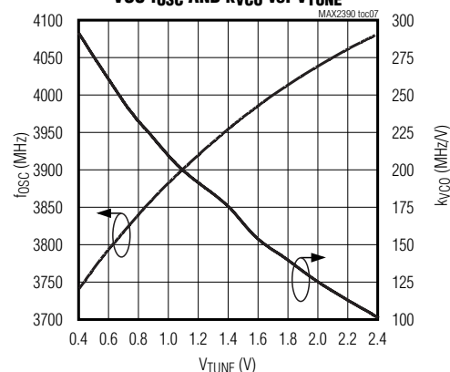
VCO f_{osc} AND k_{VCO} vs. V_{TUNE}
