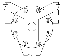
DPDT
