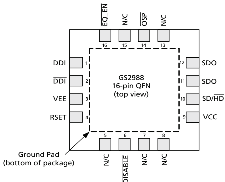
Figure 1-1: 16-Pin QFN
