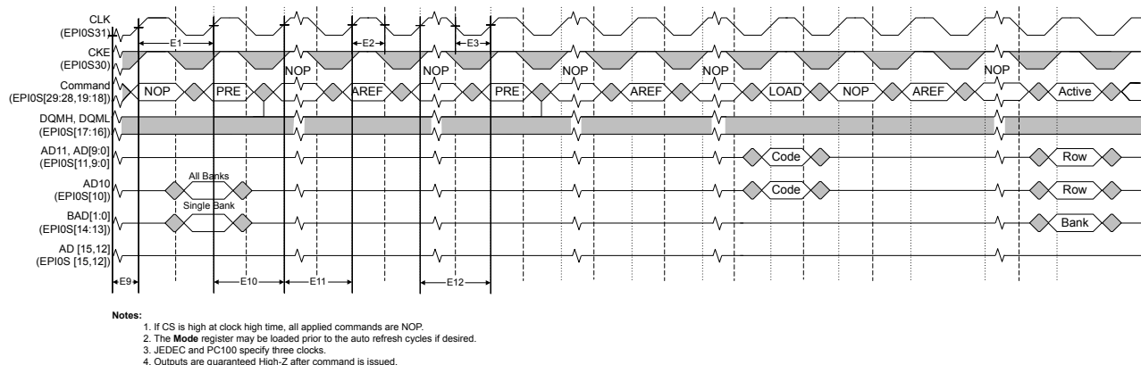
Figure 21-13. SDRAM Initialization and Load Mode Register Timing
