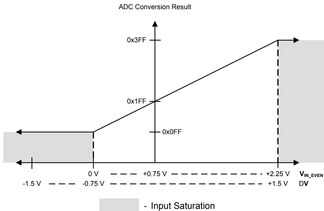
Figure 13-9. Differential Sampling Range, V_{IN\_ODD} = 2.25\text{ V}
