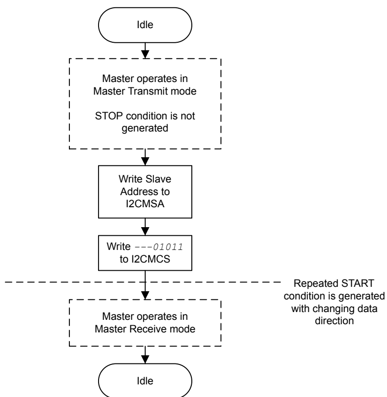
Figure 16-11. Master RECEIVE with Repeated START after TRANSMIT with Repeated START
