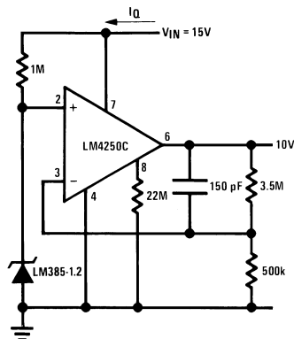
Figure 17. Micropower* 10V Reference
