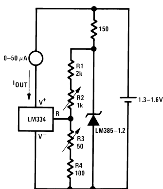
Figure 20. Lower Power Thermometer
