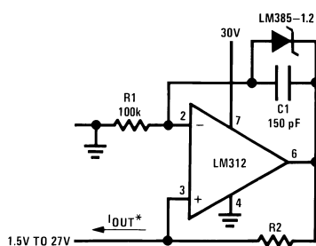
Figure 18. Precision 1μA to 1mA Current Sources
