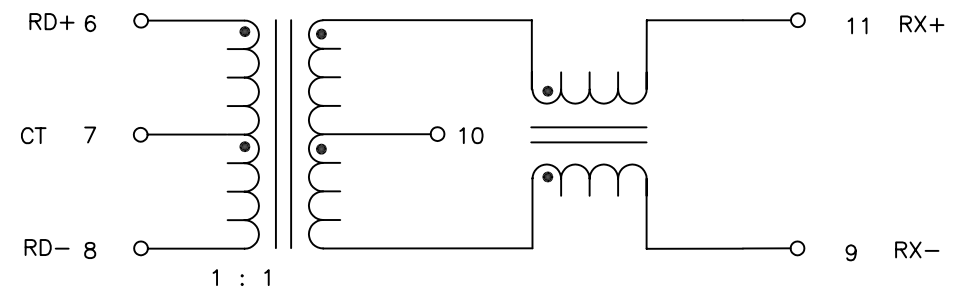
SCHEMATIC
