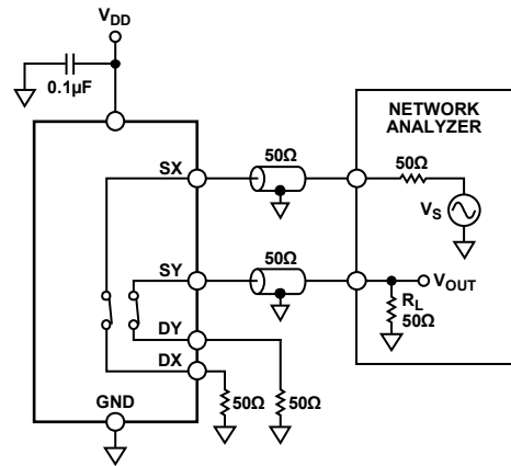
Figure 27. Channel-to-Channel Crosstalk
