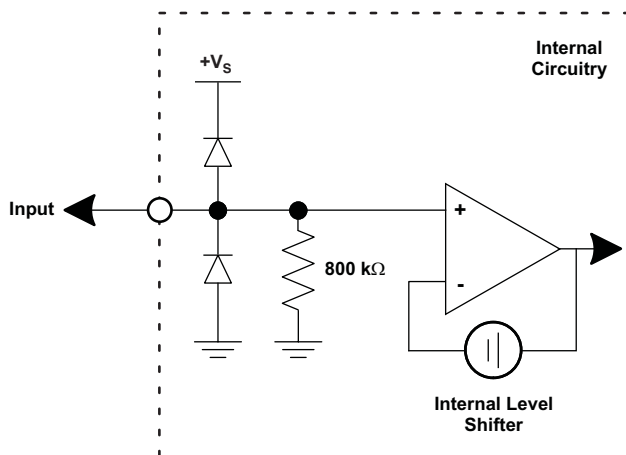
Figure 5. Equivalent DC Input Mode Circuit
