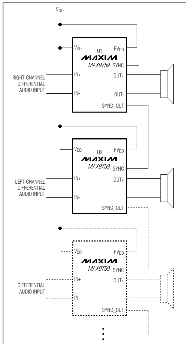
Figure 7. Master-Slave Configuration
