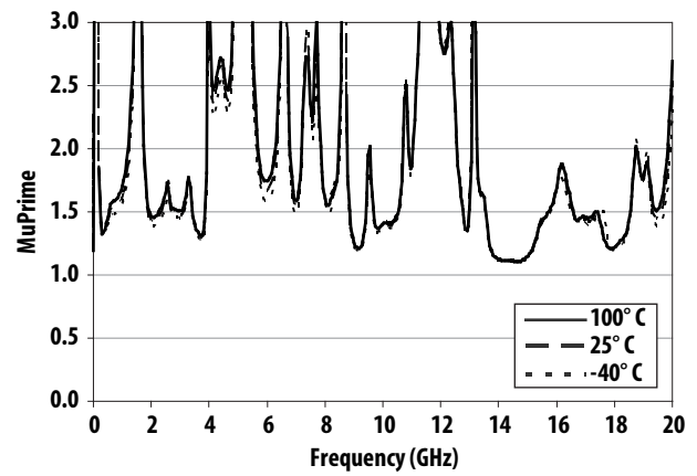
Figure 26. Mu' stability factors vs Frequency vs Temperature
