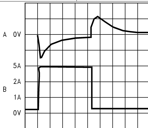
Figure 13. Discontinuous Mode Switching Waveforms, Horizontal Time Base: 1 \mu s/div
