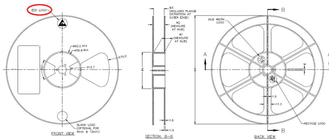
Figure 31. SOT223 reel oriented
