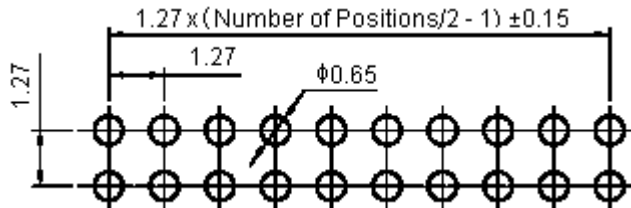
PCB Layout
