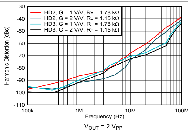
Figure 7-36. Harmonic Distortion vs Frequency
