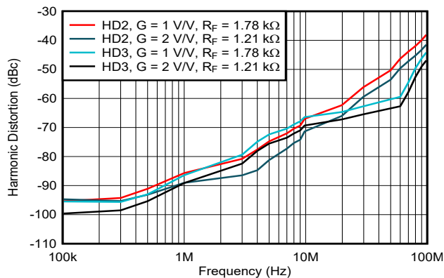
HD2 and HD3 vs Frequency at R_L = 100\text{ }\Omega
