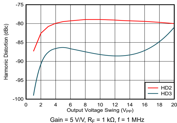
Figure 7-11. Harmonic Distortion vs Output Voltage Swing
