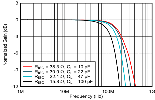
Figure 7-7. Capacitive Load Frequency Response
