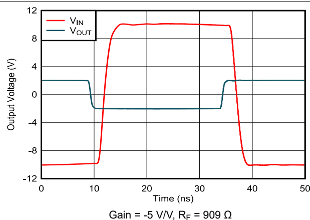
Figure 7-27. Inverting Large-Signal Transient Response
