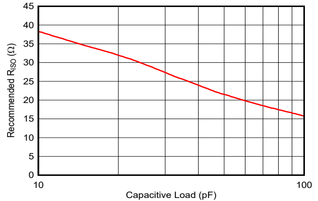
Figure 7-8. Recommended R_{ISO} vs Capacitive Load
