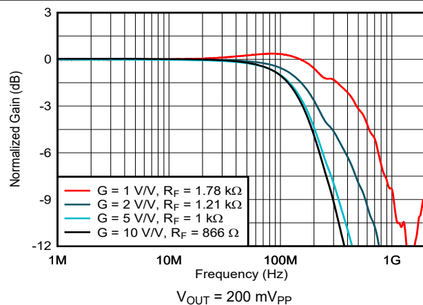
Figure 7-32. Noninverting Small-Signal Frequency Response
