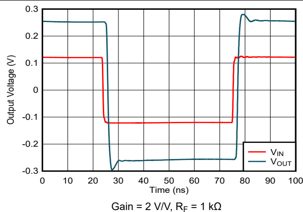
Figure 7-25. Noninverting Small-Signal Transient Response
