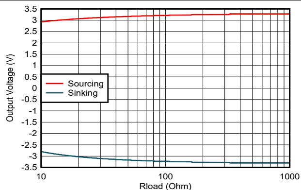
Figure 7-39. Output Voltage vs Load Resistance
