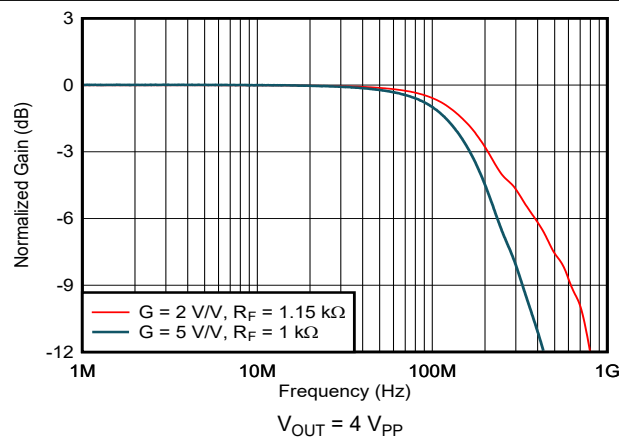
Figure 7-34. Noninverting Large-Signal Frequency Response
