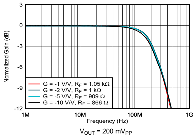
Figure 7-3. Inverting Small-Signal Frequency Response
