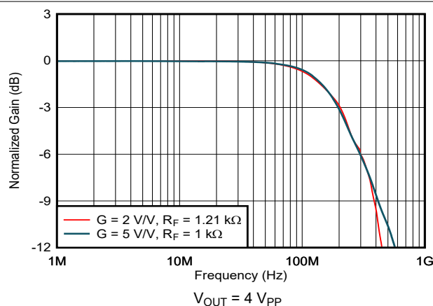
Figure 7-5. Noninverting Large-Signal Frequency Response
