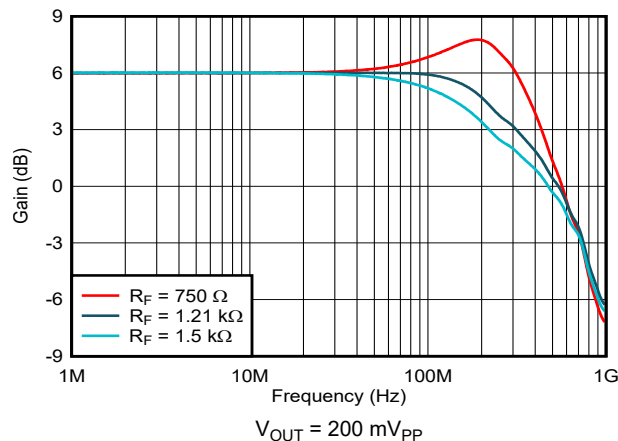
Figure 7-1. Noninverting Small-Signal Frequency Response
