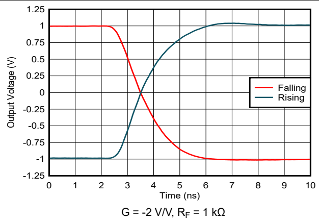
Figure 7-35. Settling Time
