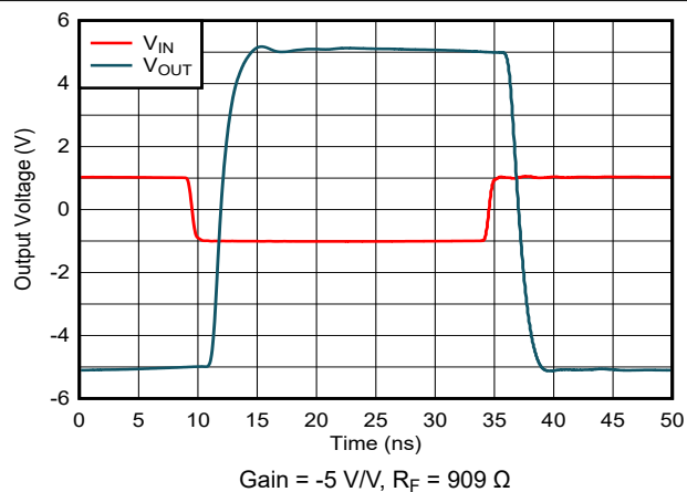
Figure 7-26. Inverting Large-Signal Transient Response
