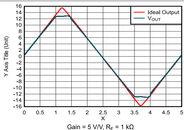
Figure 7-28. Output Overdrive Recovery Time
