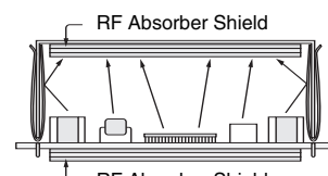
PCB Shield effectiveness can be further enhanced by adding RF absorber material under PCB (see pages 30-34).
