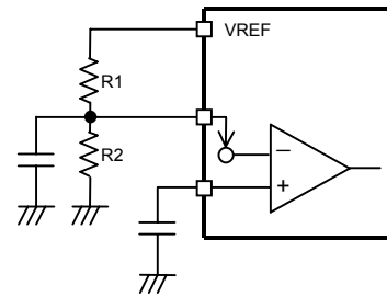
Fig.93 Soft start setting circuit
