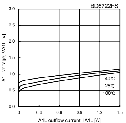
Fig.71 Low side output Body Di characteristics
