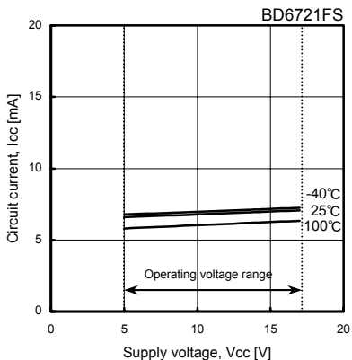
Fig.31 Circuit current
