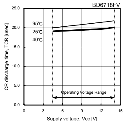
Fig.30 CR discharge time
