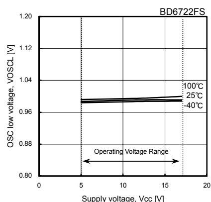
Fig.63 OSC low voltage (Voltage characteristics)
