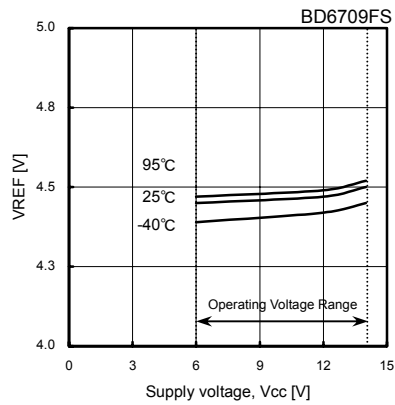
Fig.14 VREF voltage
