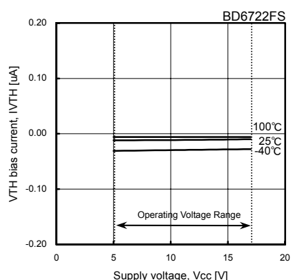
Fig.69 VTH input bias current
