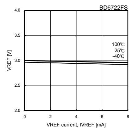
Fig.66 VREF current ability (Temperature characteristics)
