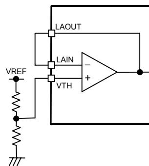
Fig.76 Level amplifier application 2
