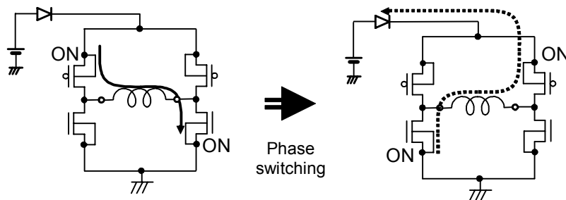
Fig.98 Vcc voltage rise by back electromotive force
