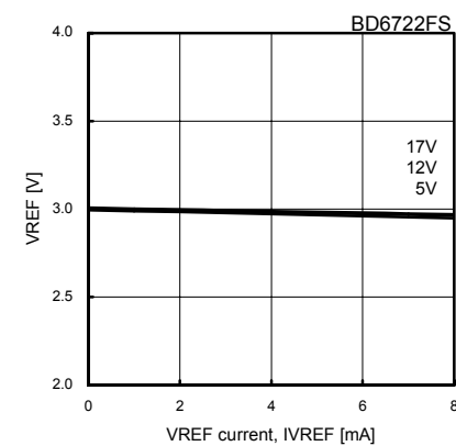
Fig.67 VREF current ability (Voltage characteristics)
