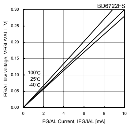
Fig.61 FG/AL low voltage (Temperature characteristics)
