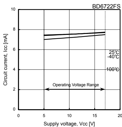
Fig.52 Circuit current
