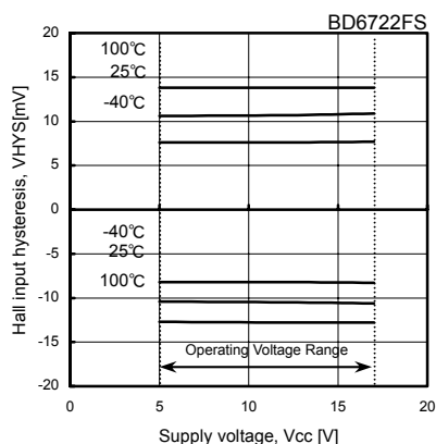
Fig.53 Hall input hysteresis
