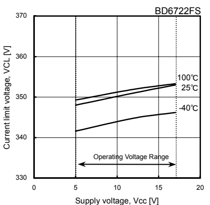
Fig.68 Current limit voltage
