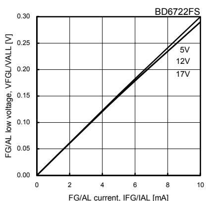
Fig.62 FG/AL low voltage (Voltage characteristics)
