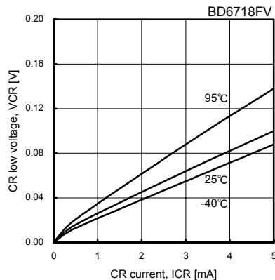
Fig.29 CR output low voltage
