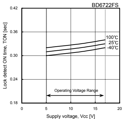
Fig.58 Lock detection ON time
