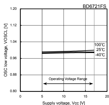
Fig.42 OSC low voltage
