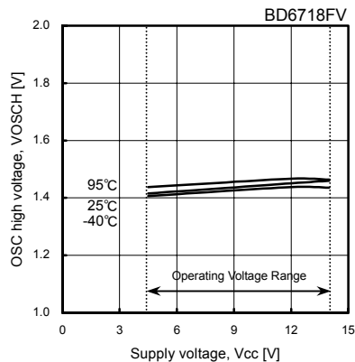
Fig.26 OSC high voltage
