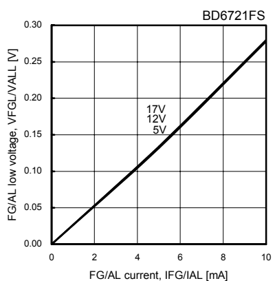
Fig.40 FG/AL low voltage (Voltage characteristics)
