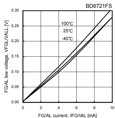
Fig.39 FG/AL low voltage (Temperature characteristics)
