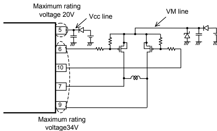
Fig.88 High voltage application (BD6722FS)
