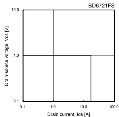
Fig.51 Output Tr ASO (upper and lower total) (TON=100msec)
