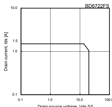
Fig.72 Low side output Tr ASO (TON=100msec)
