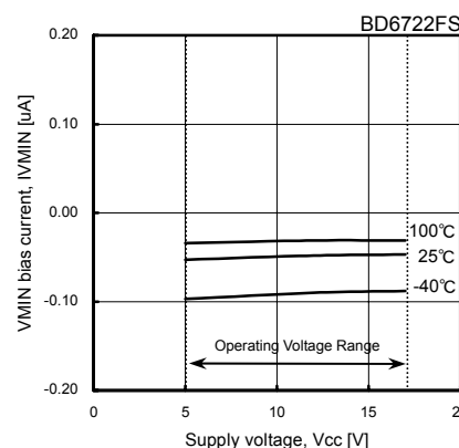
Fig.70 VMIN input bias current
