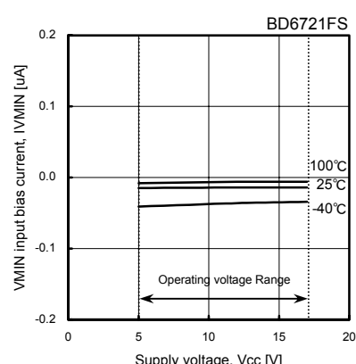
Fig.48 VMIN input bias current
