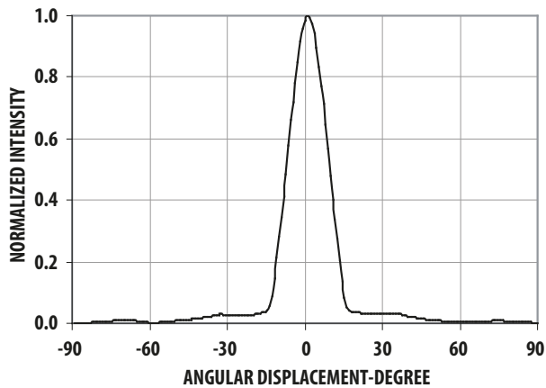
Figure 5. Radiation Pattern for 15° Viewing Angle Lamp
