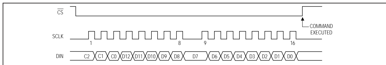
Figure 6. Serial-Interface Timing
