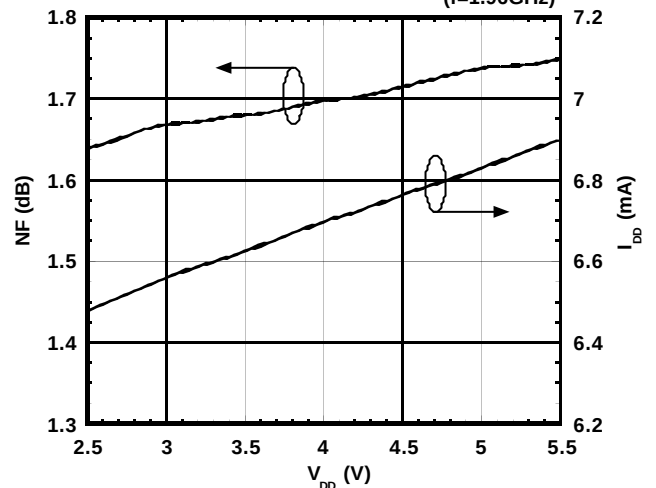
NF, I_{DD} vs. V_{DD} ( f=1.96GHz )
