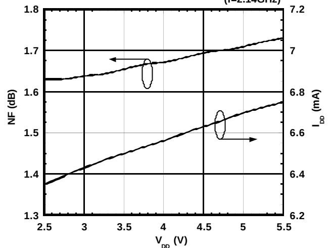
NF, I_{DD} vs. V_{DD} (f=2.14GHz)
