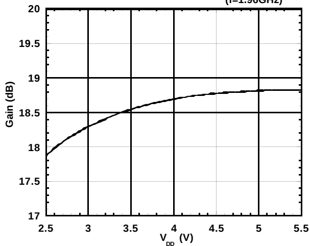
Gain vs. V_{DD} ( f=1.96GHz )
