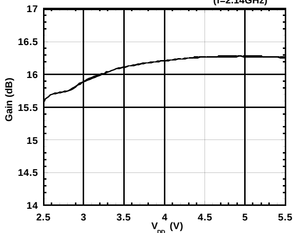
Gain vs. V_{DD} (f=2.14GHz)
