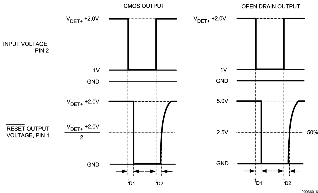
FIGURE 1. Propagation Delay Timing Diagrams
