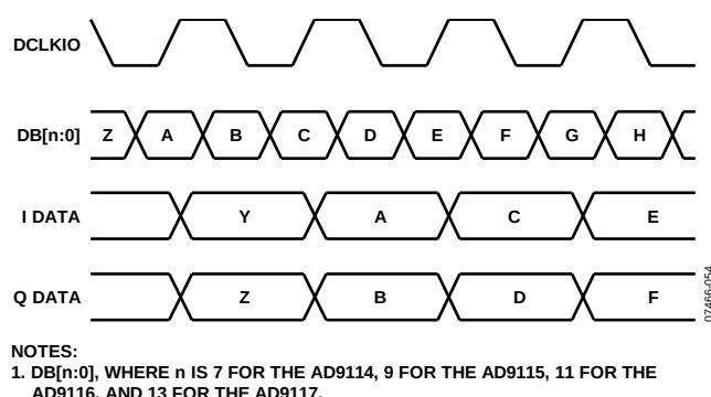
Figure 92. Timing Diagram with IFIRST = 1, IRISING = 1
