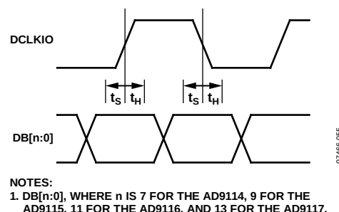
Figure 93. Setup and Hold Times for All Input Modes
