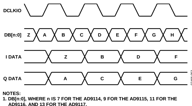
Figure 91. Timing Diagram with IFIRST = 1, IRISING = 0
