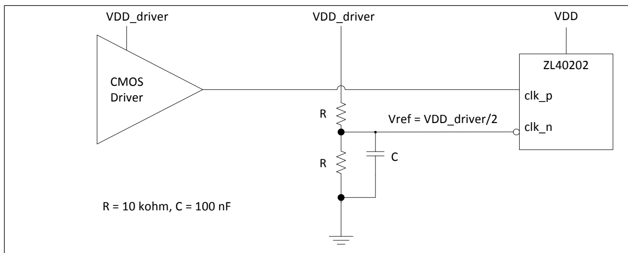
Figure 10 - CMOS Input DC Coupled Referenced to VDD/2
