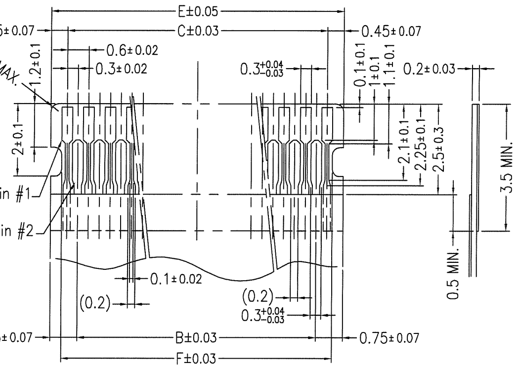
RECOMMENDED FPC CONFIGURATION
