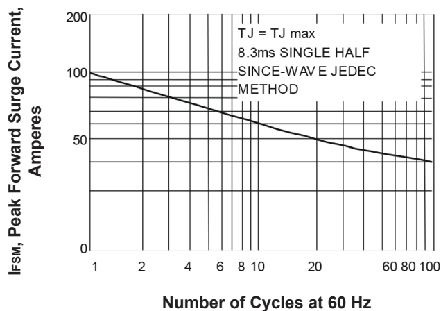
Fig. 5-Max. Non-Repetitive Peak Forward Surge Current
