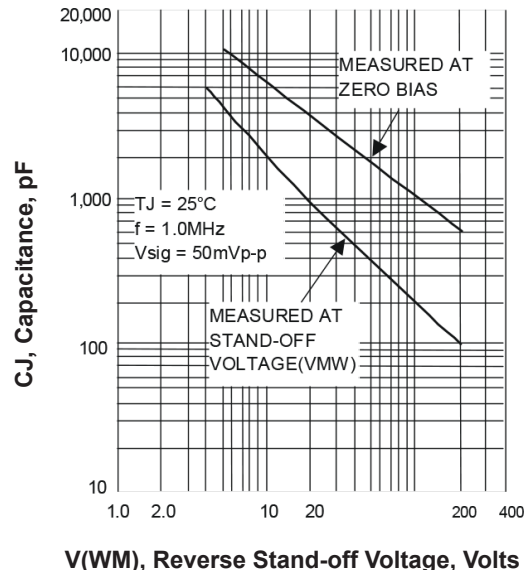
Fig. 4-Typical Junction Capacitance
