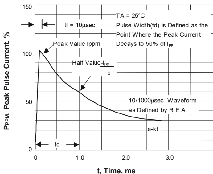
Fig. 3-Pulse Waveform
