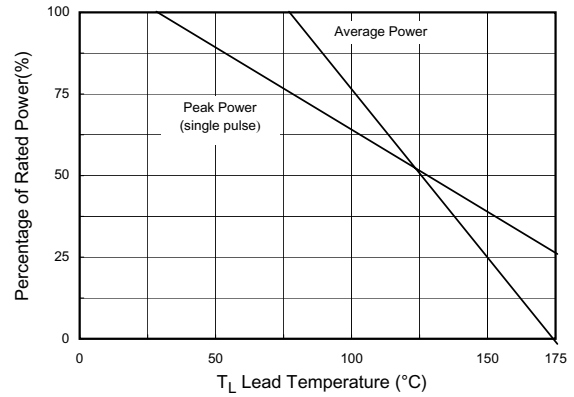
Fig.2-Power Derating Curve
