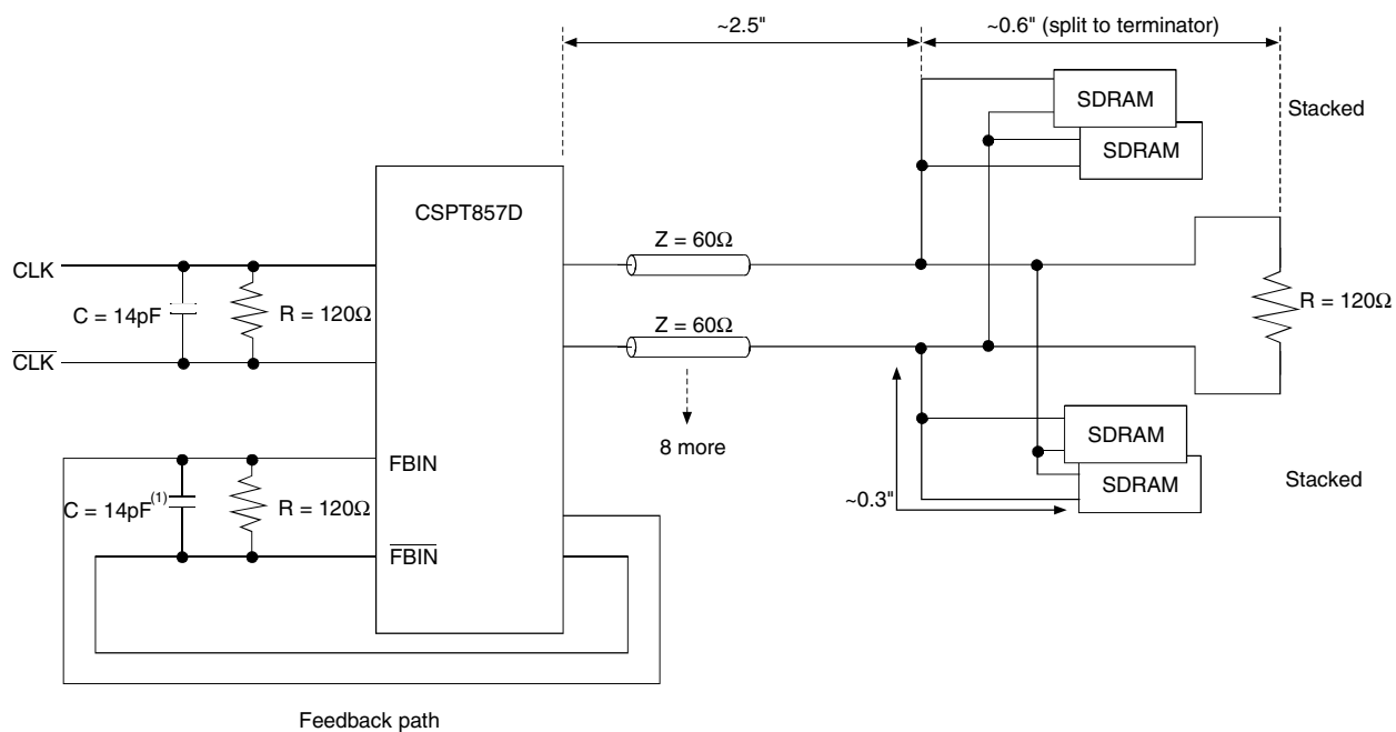
Figure 10. Clock Structure 2
