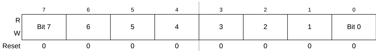
Figure 15-14. TPM Channel Value Register Low (TPMxCnVL)
