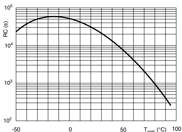
Insulation resistance as a function of the ambient temperature (typical curve)
