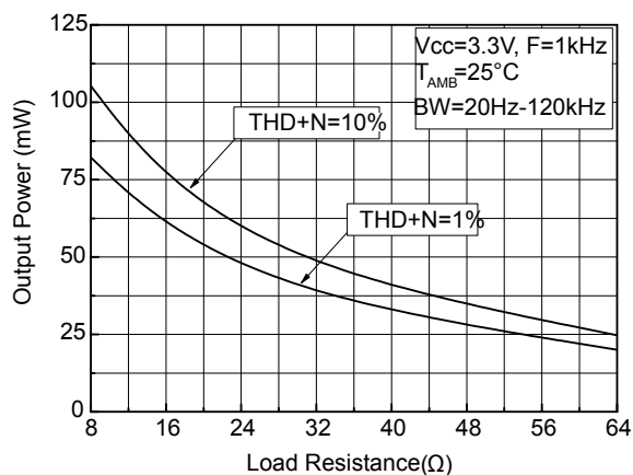
Figure 53. Output power vs. load resistance V_{CC}=3.3\ \text{V}
