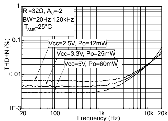
Figure 47. Total harmonic distortion plus noise vs. frequency R_L=32\ \Omega , A_V=-2
