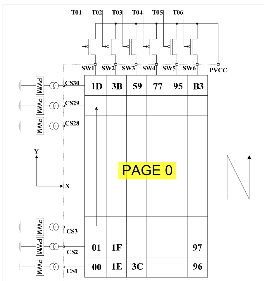
Figure 9 PWM Register
