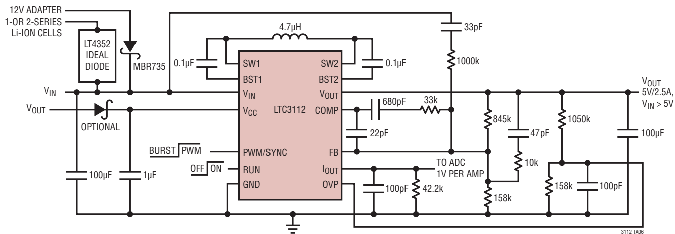
Adapter Plug-In
