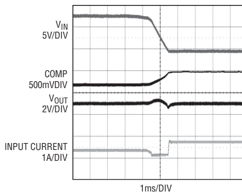
Adapter Disconnect
