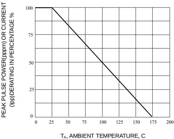
Fig. 2-PULSE DERATING CURVE
