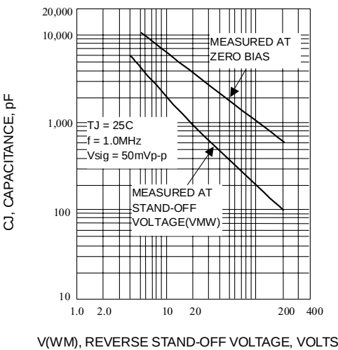
Fig. 4-TYPICAL JUNCTION CAPACITANCE
